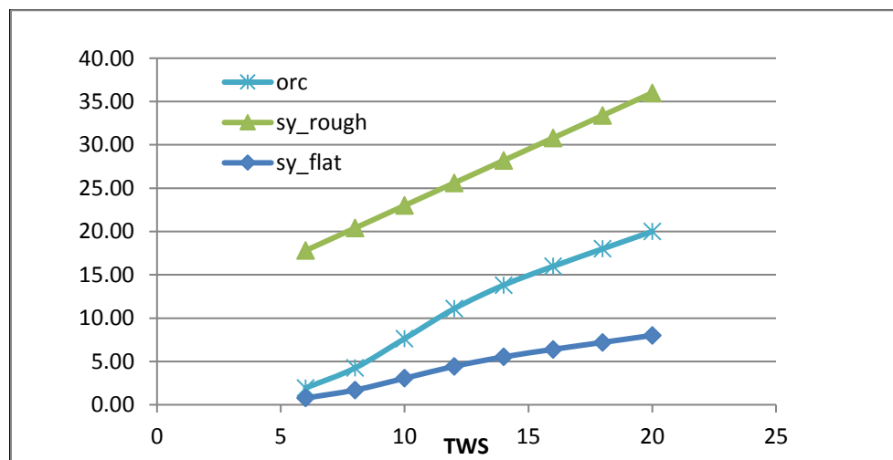
Figure 5: ORC and SY true wind speed behavior of the added resistance in waves.
